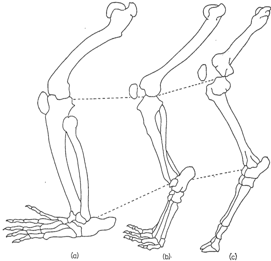
Fig. 4. Hindlimb skeletons of (a) a plantigrade, (b) a digitigrade, and (c) an unguligrade mammal to show the changes in proportions of limb segments with change of stance.
