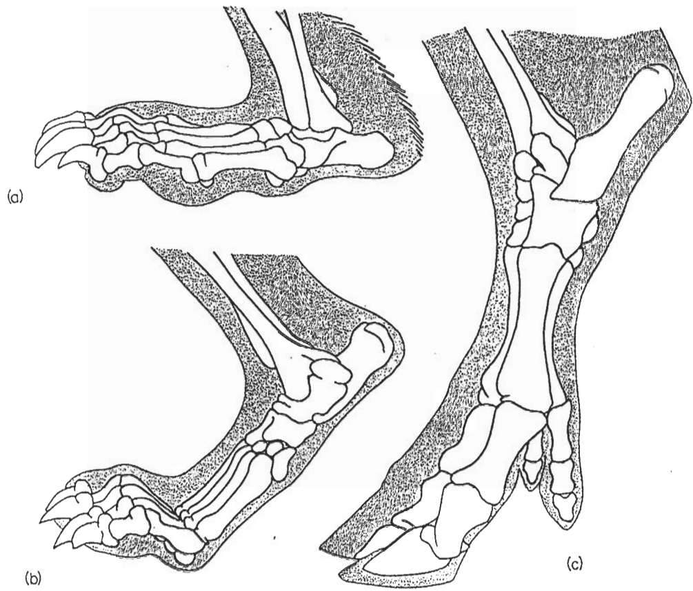
Fig. 3. The three categories of stance: (a) plantigrade (bear); (b) digitigrade (dog); (c) unguligrade (pig). After Howell, 1944.
