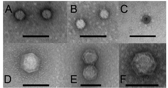
FIG 2 Transmission electron micrographs of negatively stained phages, showing their icosahedral tailless nature: φ12:2 (A), φ18:4 (B), φ12a:1 (C), φ3:2 (D), φ46:2 (E), φ48:2 (F). Scale bars equal 100 nm.
