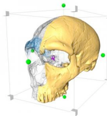
3D reconstruction of a Neandertal based on a CT-scan of the original skull (found in 1909 in La Ferrassie, Dordogne and housed in the Musée de l'Homme, Paris). Small hidden details like the inner ear (purple) can be studied without harming the original and distortions can be reconstructed with the help of computer software. (Credit: Department of Human Evolution, Max Planck Institute for Evolutionary Anthropology)
