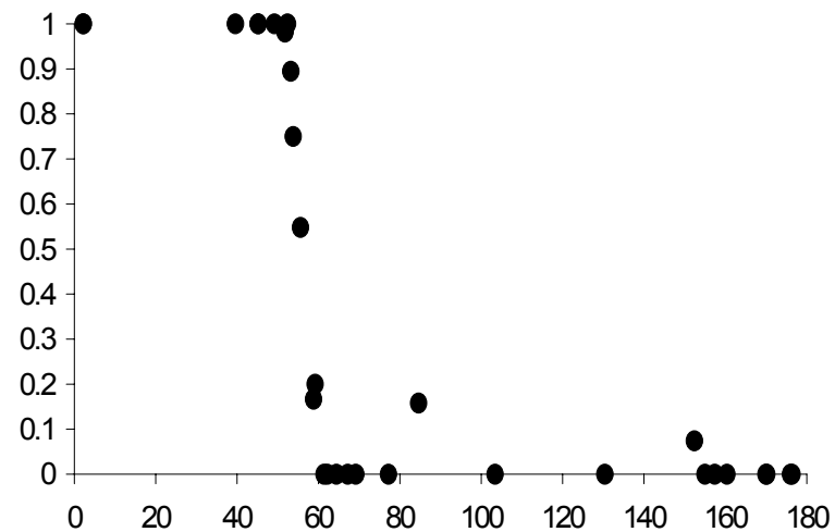
Foxp3
