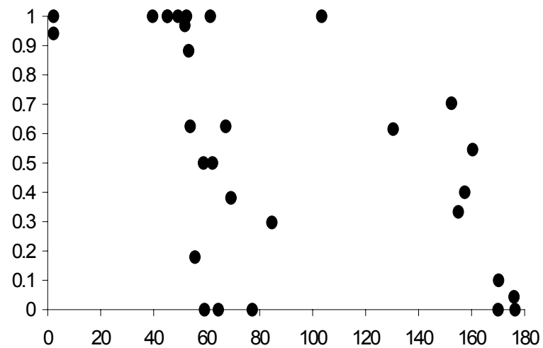
Xist
