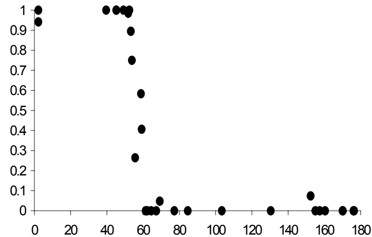
Fmr1
