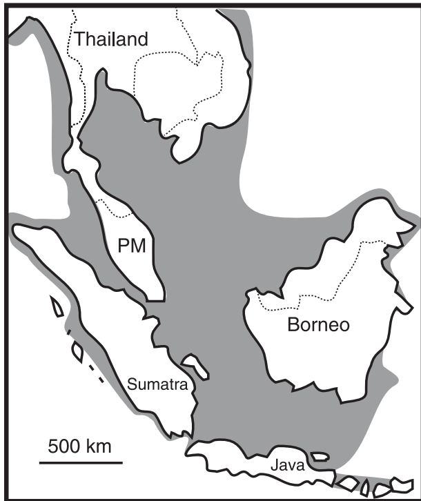
Fig. 1 Map of the Sunda region. Shading represents the additional 1.53 million km 2 of terrestrial habitat exposed when sea levels dropped to \geq 120 m below present levels during Pleistocene glacial cycles (after Vorris 2000). PM, Peninsular Malaysia.
